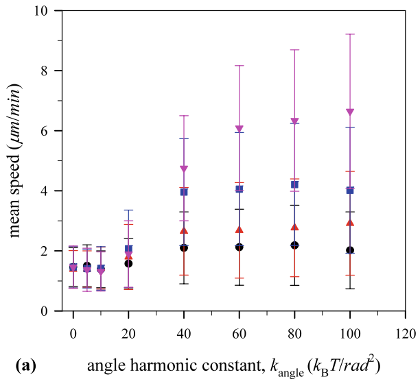
Fig. 8 (Color online) Mean speed of the model lamellipodium during simulation runs for different angle harmonic constant k_{\text{angle}} with the number of polymerization sites (a) M_p = 3 and (b) M_p = 21 . Notations are the same as in Fig. 6
