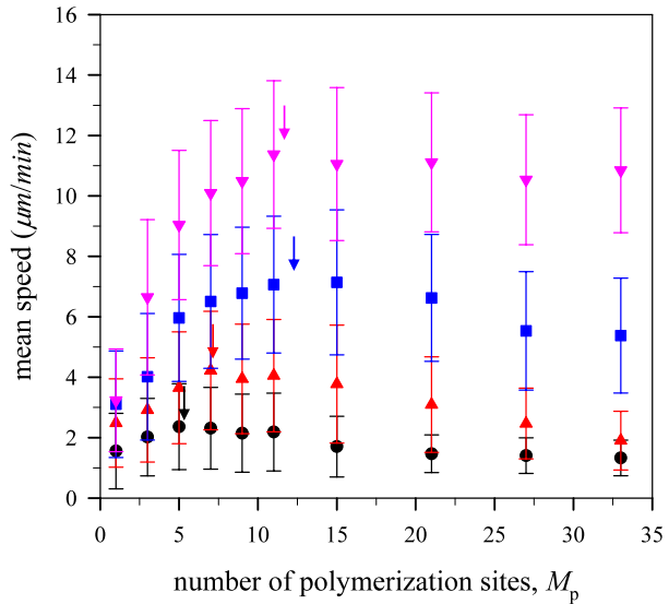
Fig. 6 (Color online) Mean speed of the model lamellipodium during simulation runs for different number of polymerization sites with harmonic angle constant k_{\text{angle}} = 100 k_B T / \text{rad}^2 at different G-actin monomer concentration c = 24 \mu\text{M} (●), 48 \mu\text{M} (▲), 96 \mu\text{M} (■), and 192 \mu\text{M} (▼)
