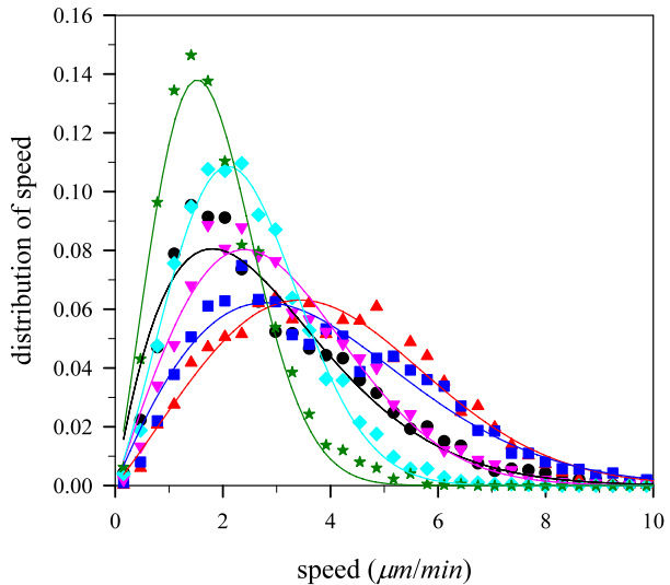
Fig. 9 (Color online) Distribution of the model lamellipodium speed at G-actin monomer concentration c = 48 \mu\text{M} with angle harmonic constant k_{\text{angle}} = 100 k_B T/\text{rad}^2 at various number of polymerization sites, M_p . Notations are the same as in Fig. 4
