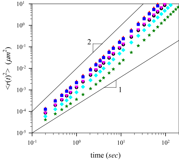
Fig. 5 (Color online) Mean-square displacement of the center of mass of the model lamellipodium during simulation runs for different number of polymerization sites with angle harmonic constant k_{\text{angle}} = 100 k_B T / \text{rad}^2 at G-actin monomer concentration c = 48 \mu\text{M} . The solid lines with slopes 1 and 2 are shown to demonstrate two different asymptotic regimes with diffusive and ballistic motion, respectively. Notations are the same as in Fig. 4
