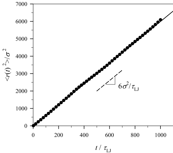
Fig. 3 Mean-square displacement of particles during simulation runs at monomer concentration c = 0.001\sigma^{-3} , or 0.13 \mu\text{M} . The dashed and solid lines in the plot are the best-fit to the data points and the analytical solution of (5) for a single particle, respectively
