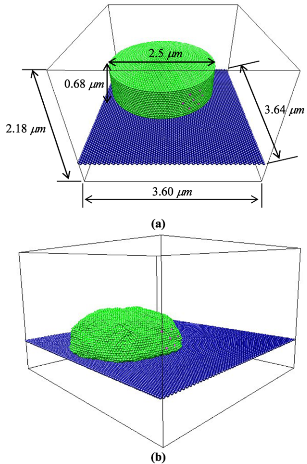
Fig. 1 (Color online) Snapshots of a virtual lamellipodium on ECM surface. Green particles represent the virtual lamellipodium, pink ones polymerization sites, and blue ones ECM surface. A virtual lamellipodium is modeled as a low-aspect-ratio doubly capped cylinder formed by wrapping a hexagonally packed sheet. F-actin filaments are firmly attached to a lamellipodium surface where polymerization sites are located, and actin polymerization takes place by connecting a G-actin particle to a polymerization site and to the first particle of a growing F-actin filament whose stiffness is given by bond angle potential. The thermal motion and stiff bond angle potential pushes the lamellipodium wall away from the F-actin filament to accommodate the added particles. The conformation of the virtual lamellipodium was relaxed (a) before the simulation run and (b) during this relaxation it assumed a bell shape
