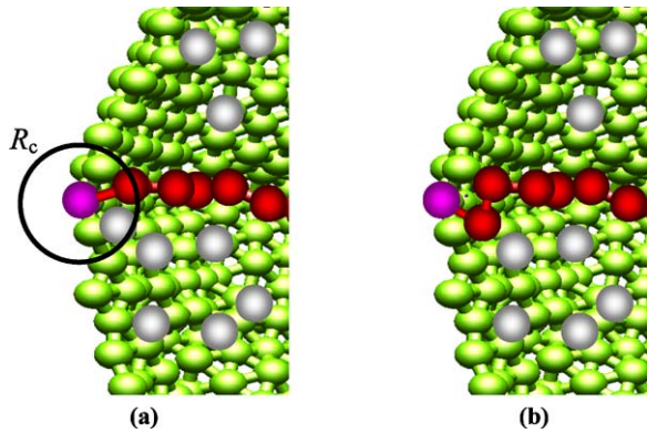
Fig. 2 (Color online) Schematic representation of the chain polymerization process: (a) particle selection and (b) bond connection. The color code is as follows: cell—green; G-actin particles—gray; F-actin filaments—red; polymerization sites—pink. Used system parameters in this figure are as follows: angle harmonic constant is k_{\text{angle}} = 0 \text{ k}_B T / \text{rad}^2 (flexible actin filament) and the number of polymerization sites, M_p = 1
